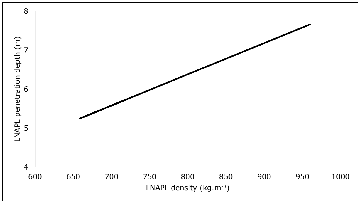
Figure A4-2. Sensitivity of LNAPL penetration depth to LNAPL density
