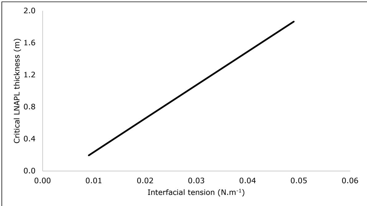
Figure A4-7. Sensitivity of LNAPL critical thickness to interfacial tension
