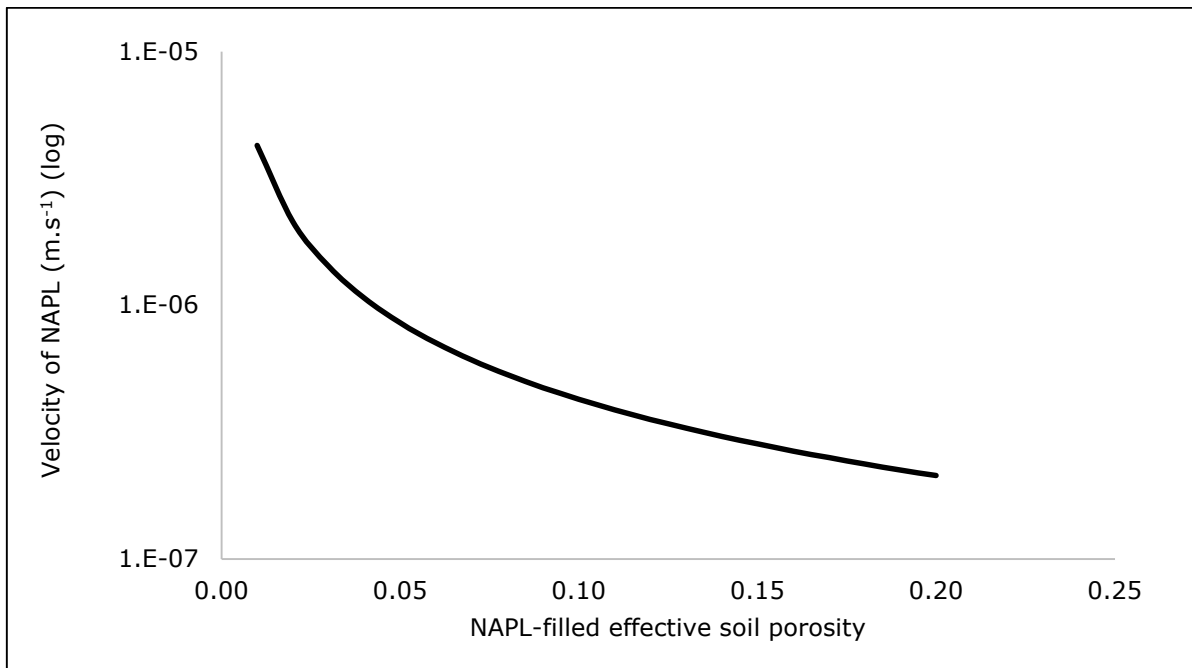
Figure A4-14. Sensitivity of velocity of LNAPL to Darcy flux for LNAPL-filled effective soil porosity
