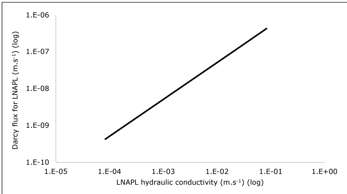
Figure A4-19. Sensitivity of LNAPL Darcy flux to LNAPL hydraulic conductivity
