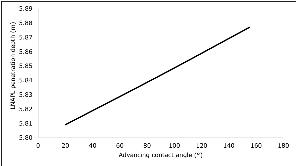
Figure A4-4. Sensitivity of LNAPL penetration depth to advancing contact angle
