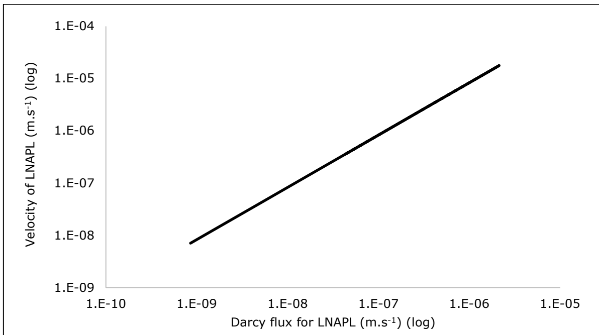
Figure A4-13. Sensitivity of velocity of LNAPL to Darcy flux for LNAPL
