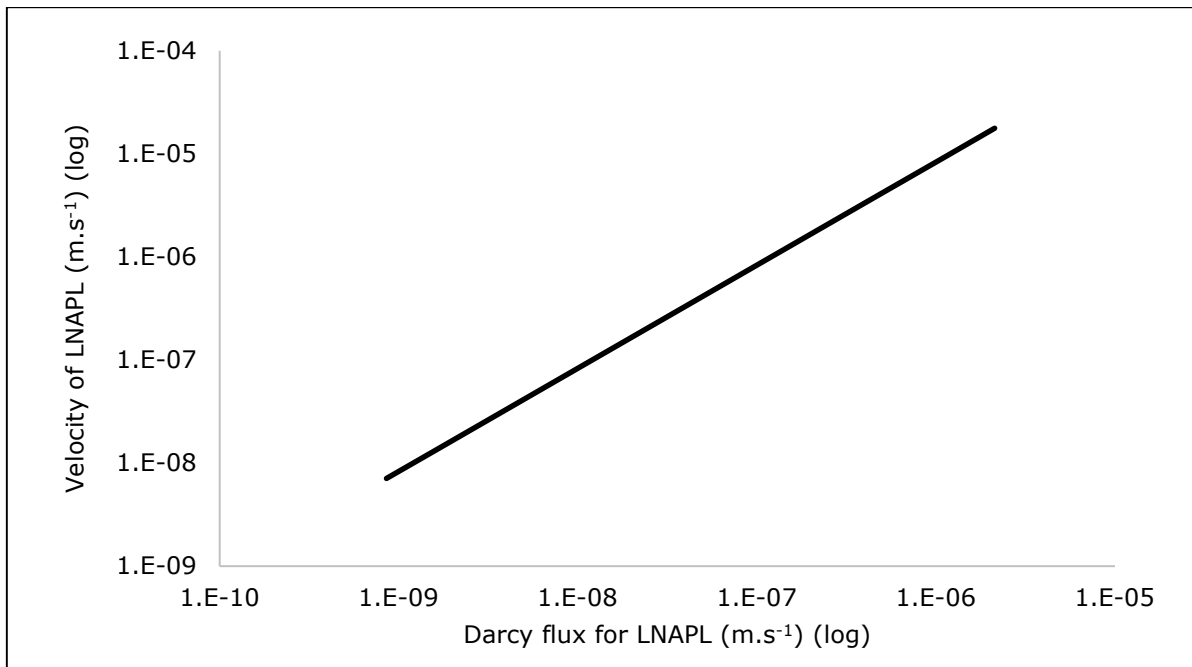
Figure A4-15. Sensitivity of velocity of LNAPL to LNAPL Darcy flux
