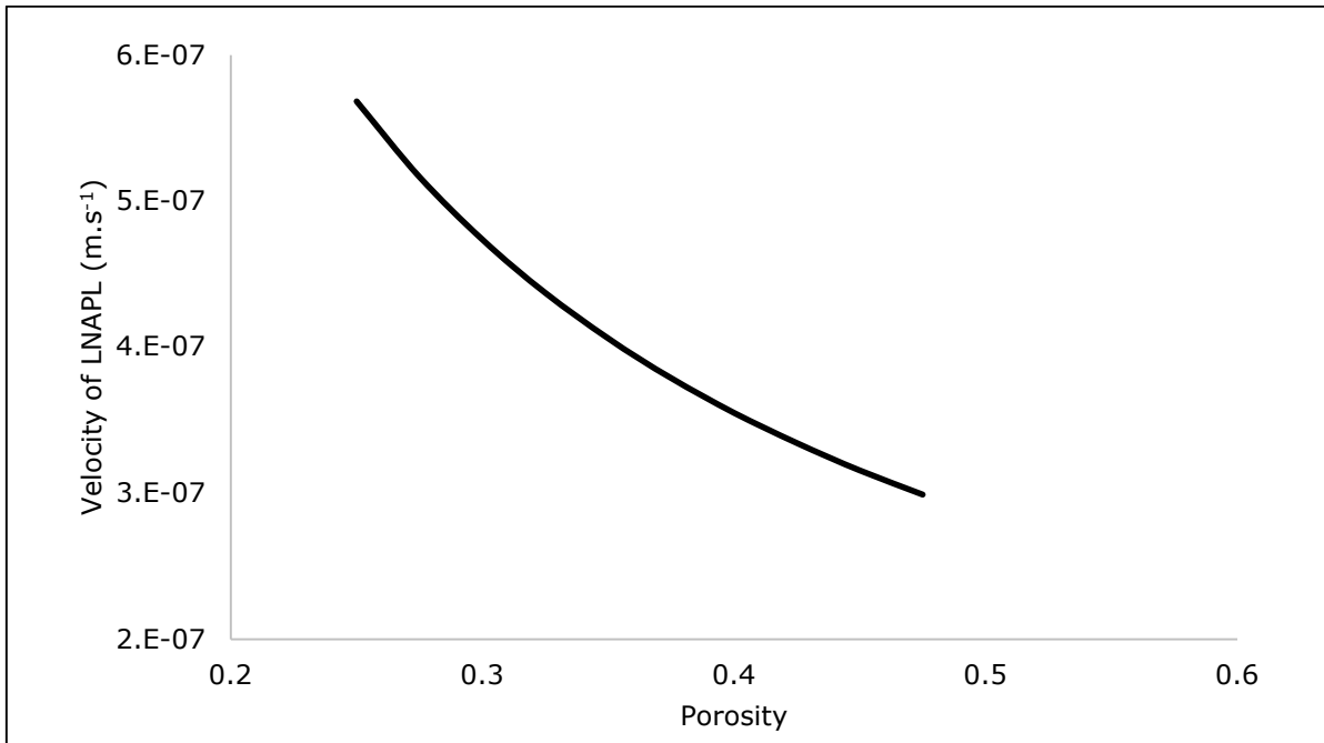
Figure A4-16. Sensitivity of velocity of LNAPL to porosity
