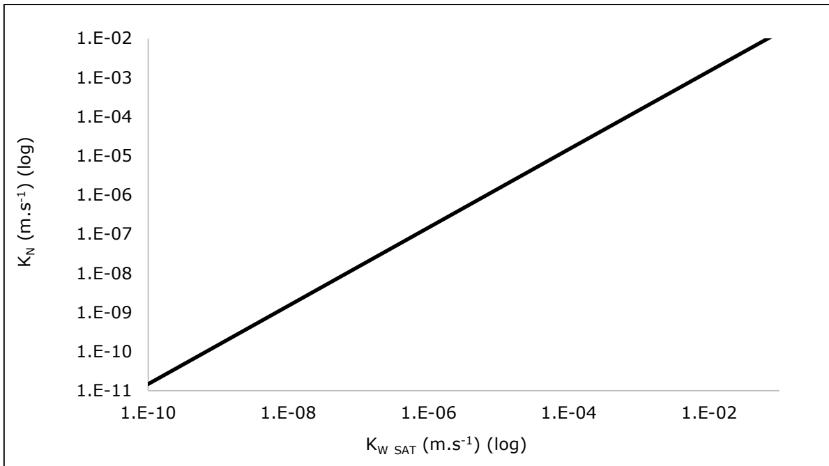
Figure A4-20. Sensitivity of LNAPL hydraulic conductivity to groundwater hydraulic conductivity
