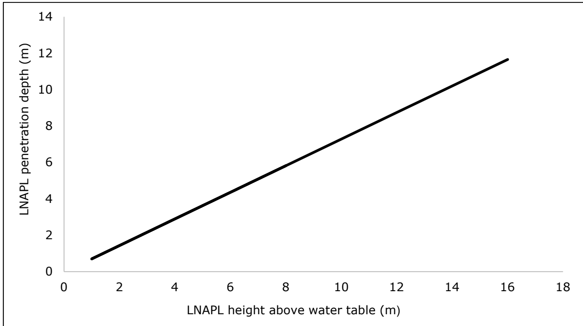
Figure A4-1. Sensitivity of LNAPL penetration depth to LNAPL height above the water table
